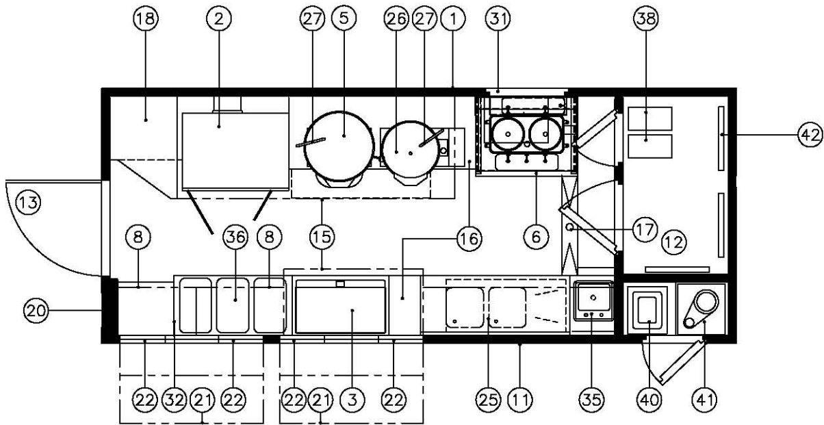
FLOOR PLAN
